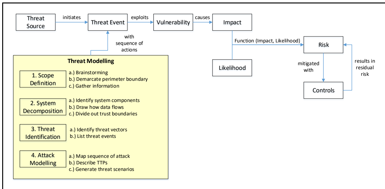
Figure 2: How Threat Modelling Fits into Risk Assessment
