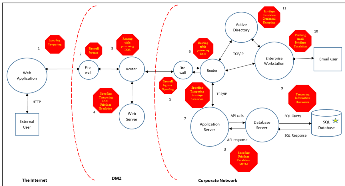
Figure 12: Complete DFD enumerated with possible threat events
