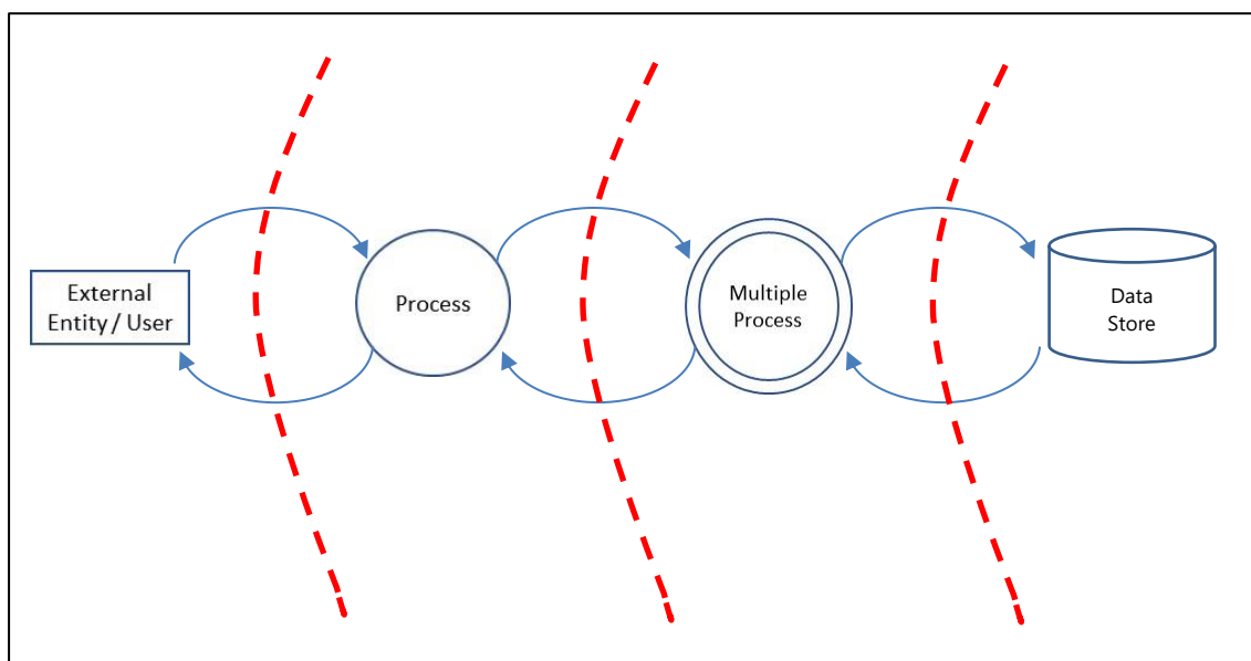
Figure 5: Example of Trust Boundaries
