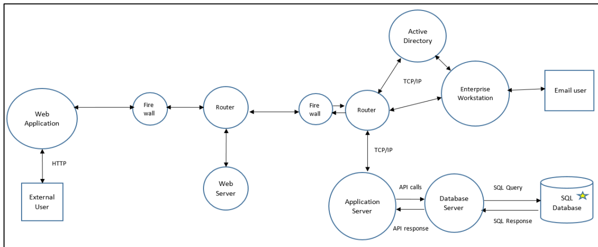
Figure 9: Data Flow Diagram
