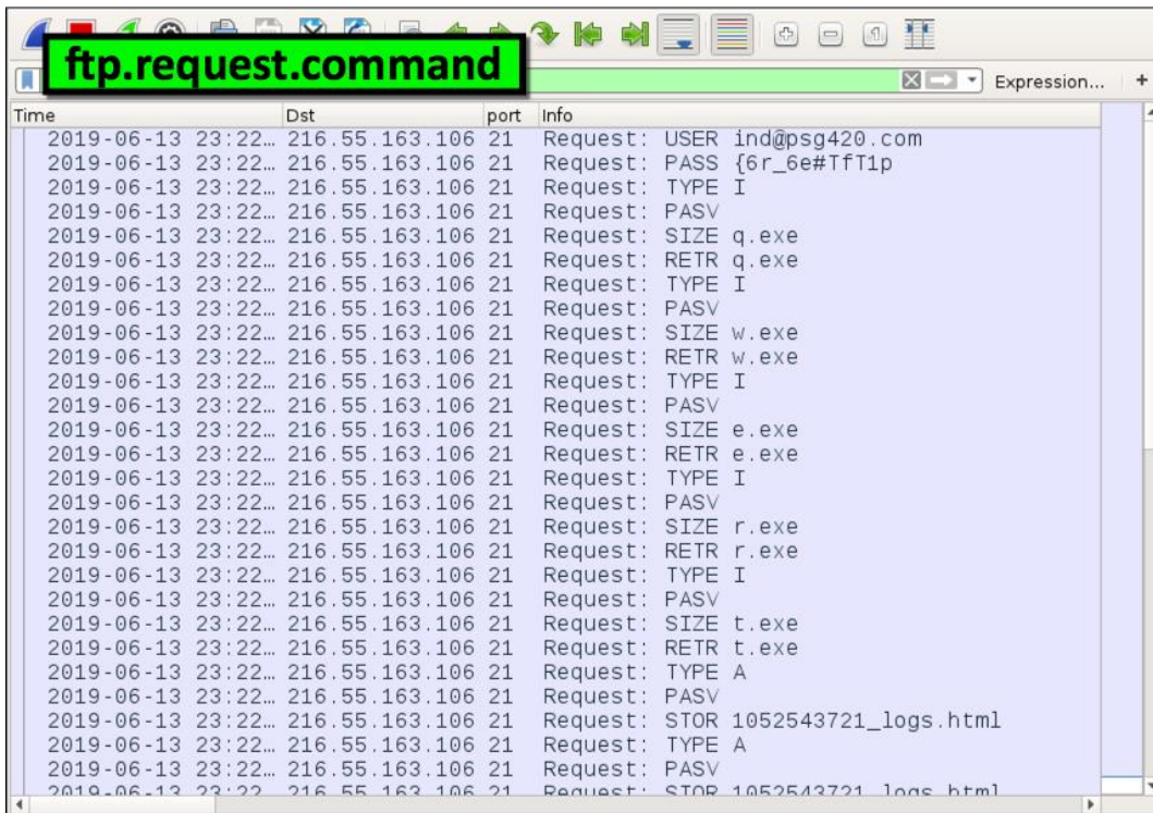
Figure 14. Filtering for FTP requests in Wireshark.
