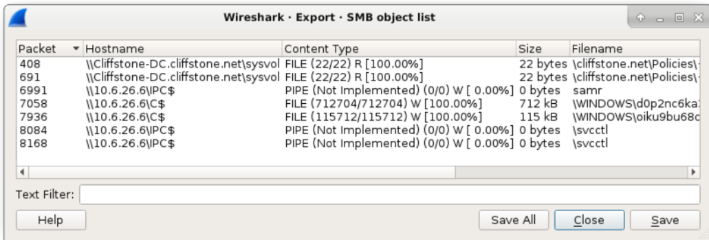
Figure 9. The export SMB object list.
