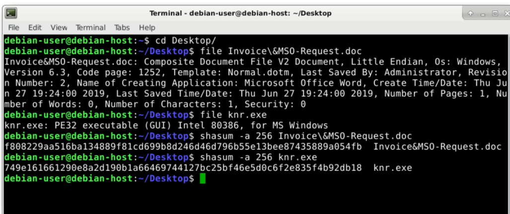
Figure 5. Determining the file type and hash of our two objects exported from the pcap.
