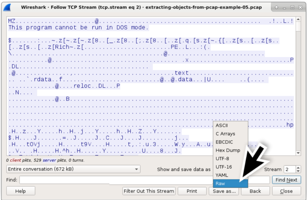
Figure 18. Selecting "Raw" from the "Show and save data as" menu.
