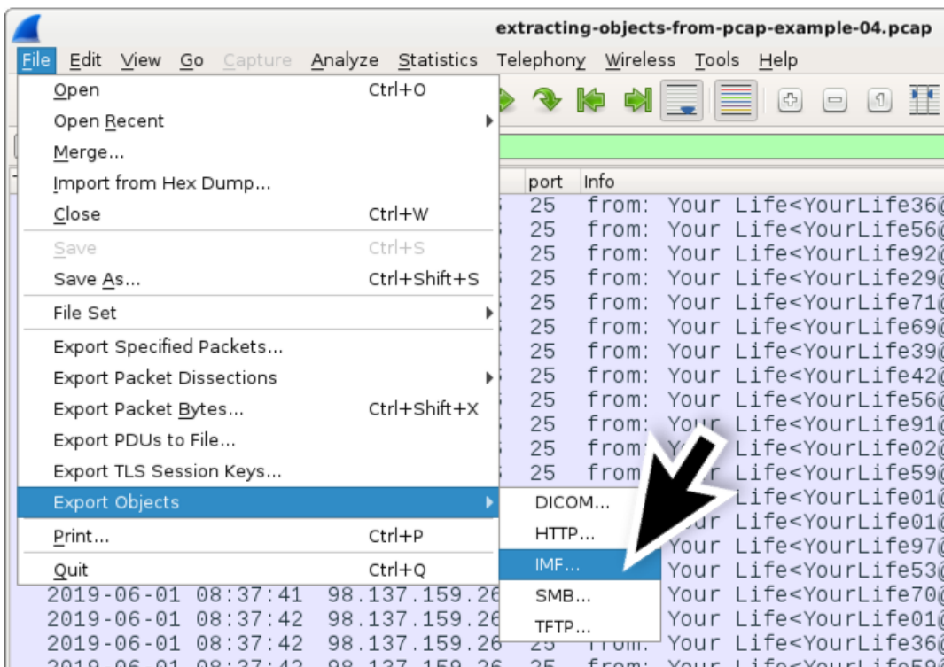
Figure 11. Exporting emails from a pcap in Wireshark.
