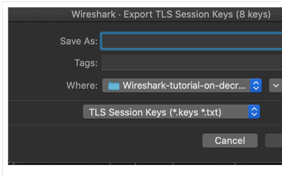
Figure 5.14. Export TLS Session Keys window
