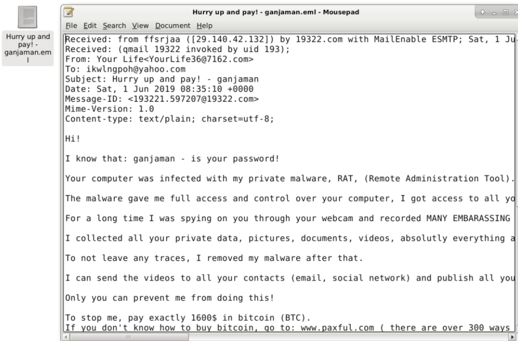
Figure 13. Using a text editor to view an .eml file exported from the pcap.
