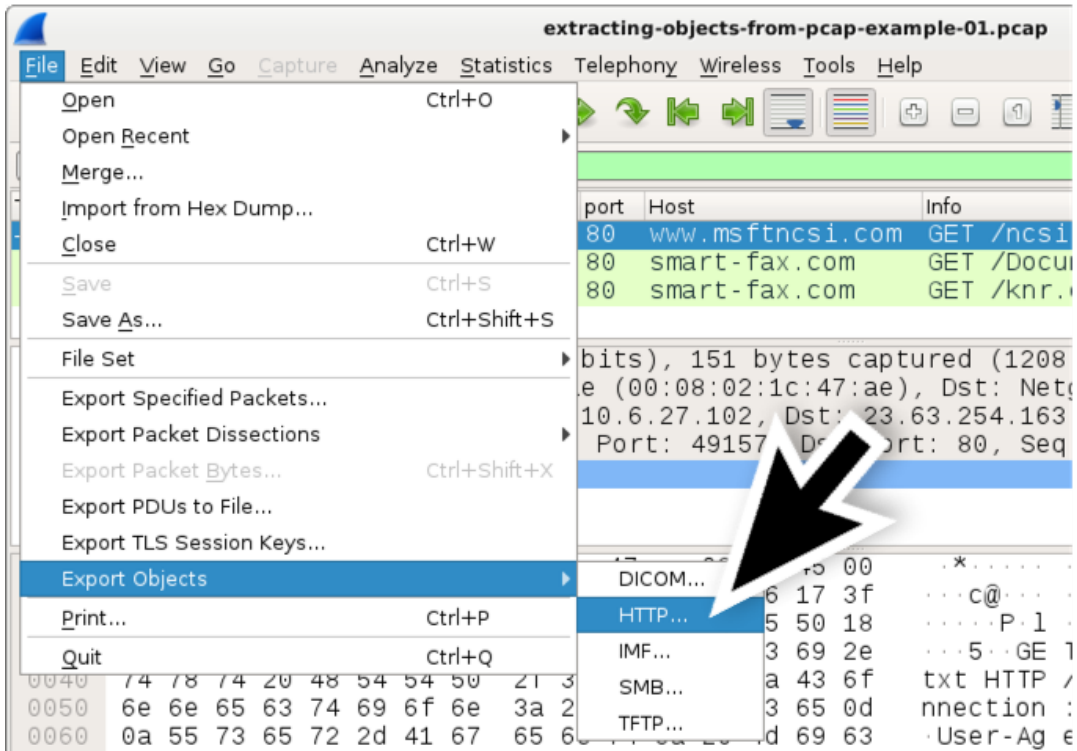
Figure 2. Exporting HTTP objects in Wireshark.
