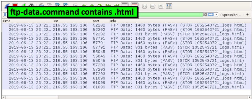
Figure 21. Filtering on files with .html in the file name over the FTP data channel.
