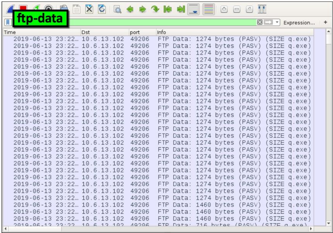
Figure 15. Filtering on FTP data traffic in Wireshark.
