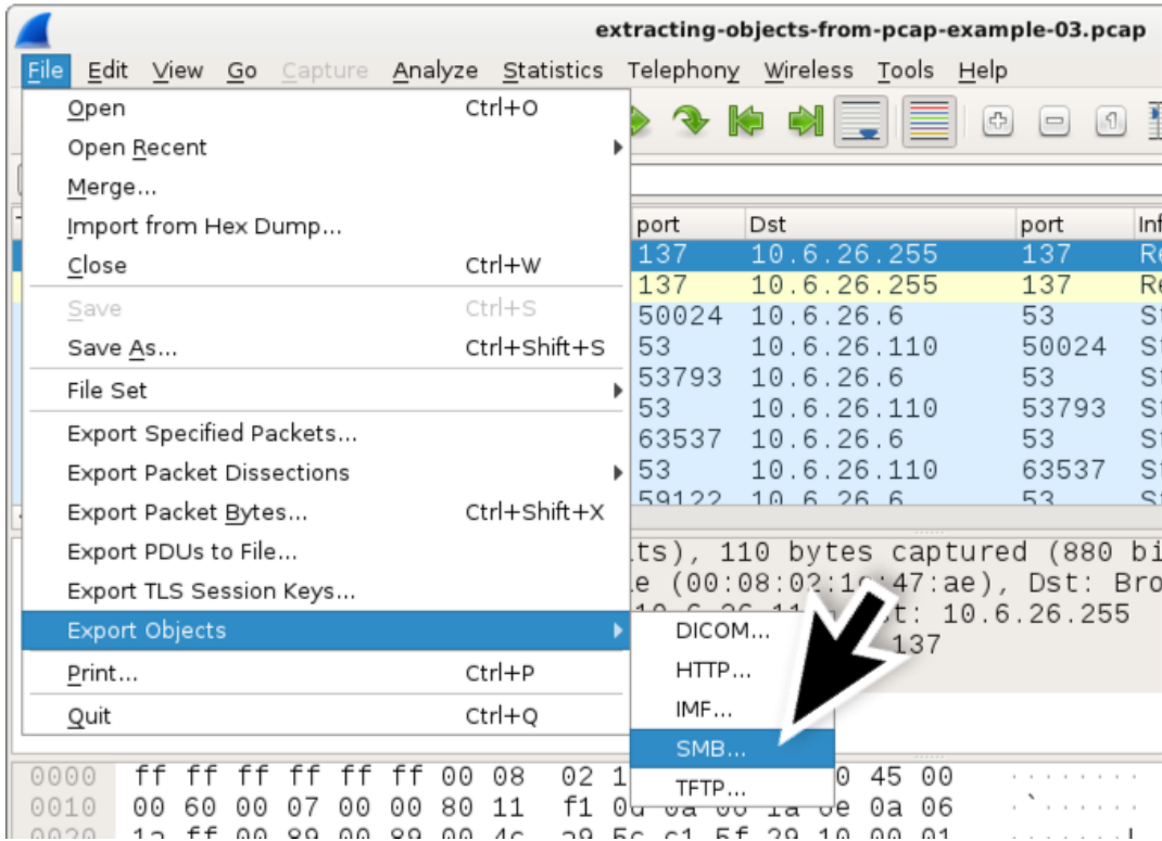
Figure 8. Getting to the Export SMB objects list.
