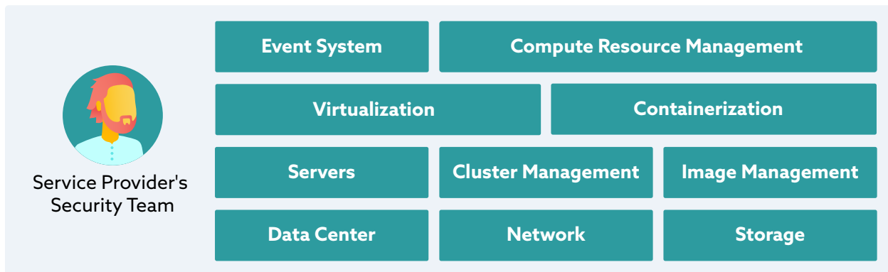
Image based Serverless shared responsibility model
