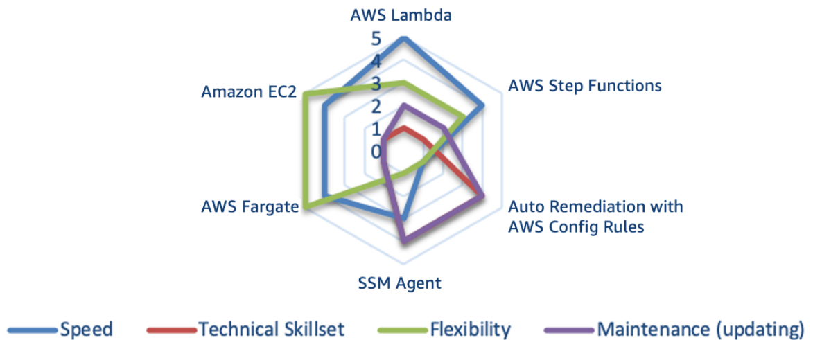
Figure 4: Differences in technical attributes across automated response approaches
