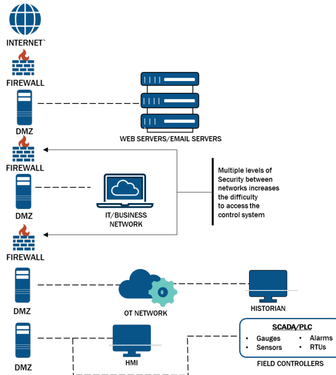
Figure 3: Network Segmentation
