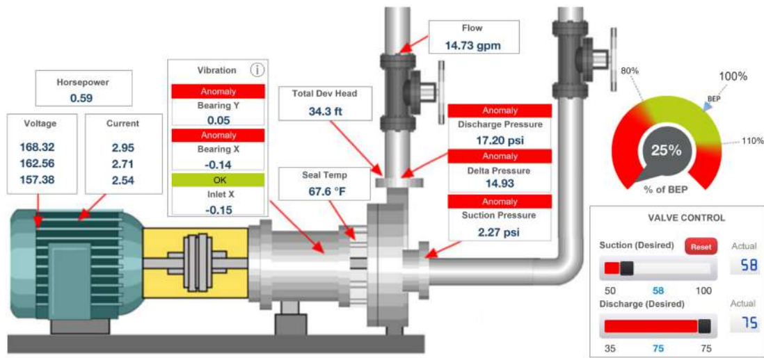
Figure 2.16: Pump monitoring solution by Flowserve [119]
