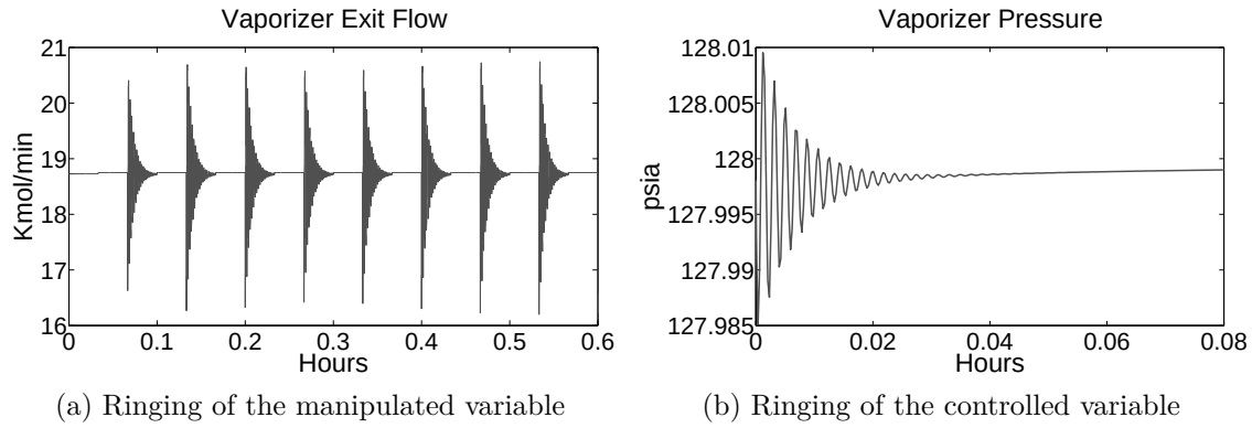
Figure 4.24: Outcome of the vaporizer exit flow valve manipulation
